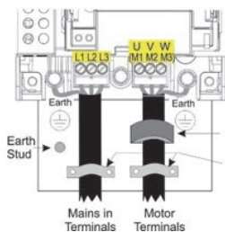
Ferrite core option to meet C2 EMC Standard Cable Clamps
